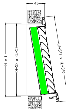
UR3: fixing with screws
