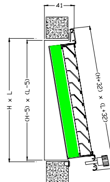
UR4: fixing with pommel
