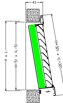
UR2: fixing with magnets
